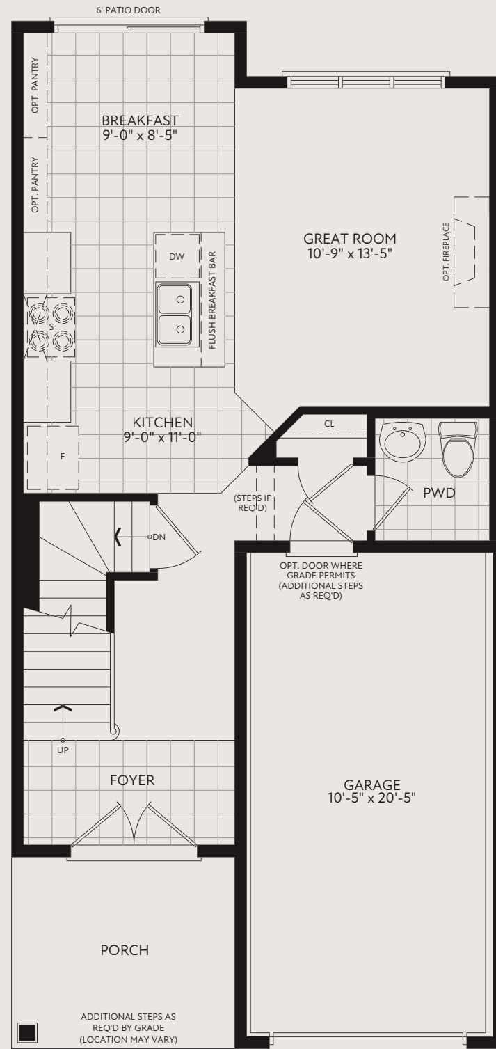
GROUND FLOOR PLAN HERITAGE
