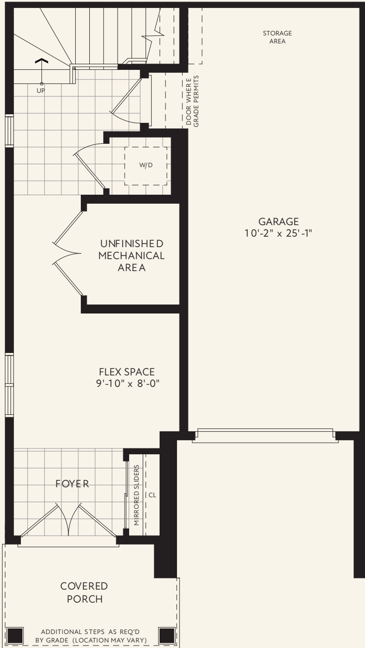
GROUND FLOOR PLAN CRAFTSMAN
