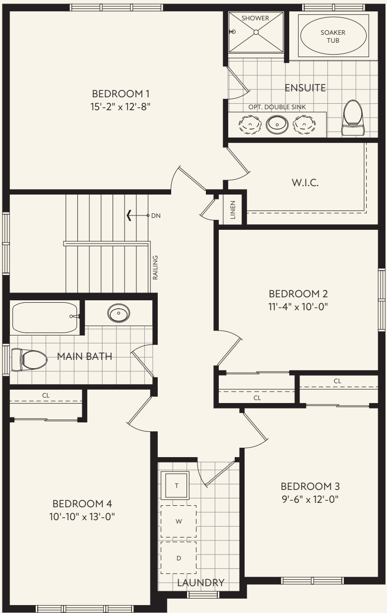
SECOND FLOOR PLAN CRAFTSMAN
