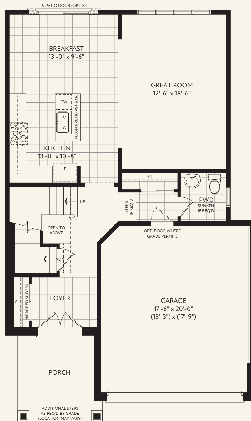
GROUND FLOOR PLAN CRAFTSMAN
