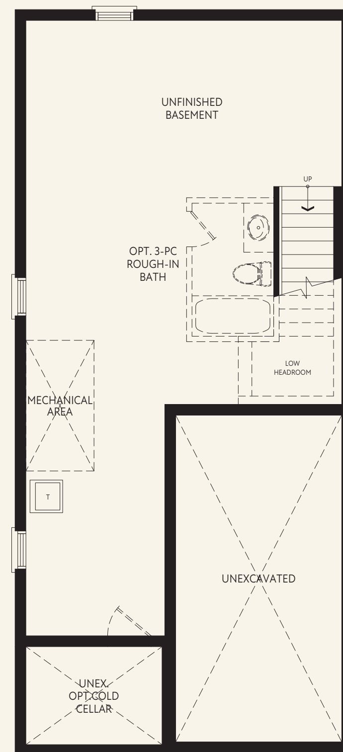
BASEMENT PLAN CRAFTSMAN
