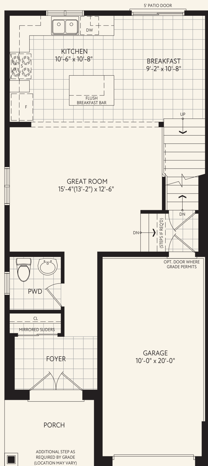
GROUND FLOOR PLAN CRAFTSMAN
