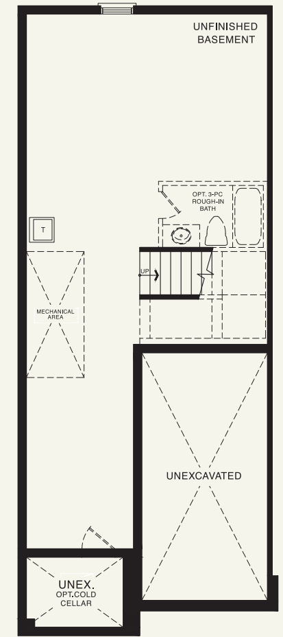
BASEMENT PLAN STYLE A1
