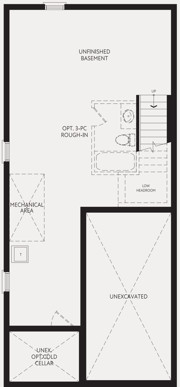
BASEMENT PLAN CRAFTSMAN
